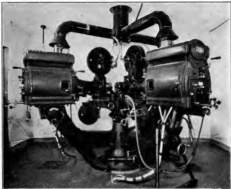
FIG. 1. Rear view, showing lateral panning screw at bottom of base; also swiveled exhaust pipes overhead.
